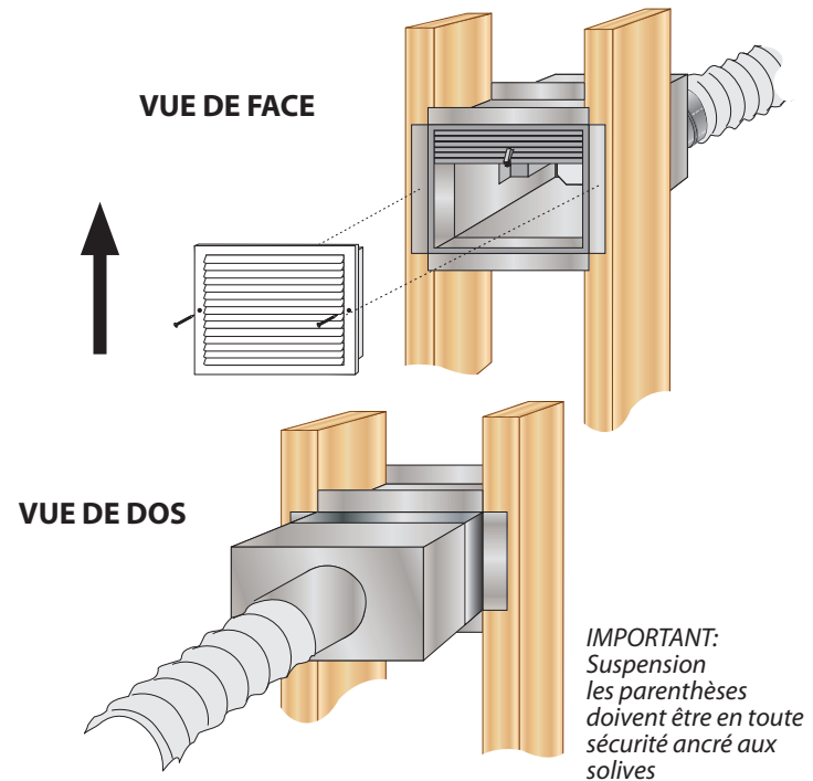
FIGURE 1 - MONTAGE
