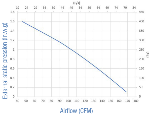
EK150-TQG Ventilation Performance
