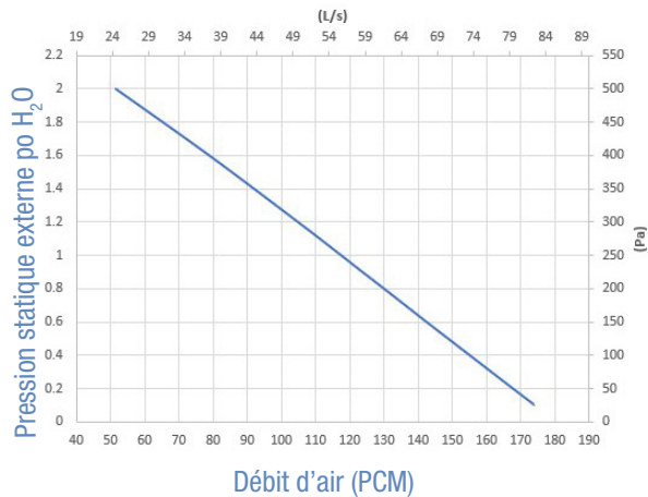
EK150-TQX Performance de ventilation
