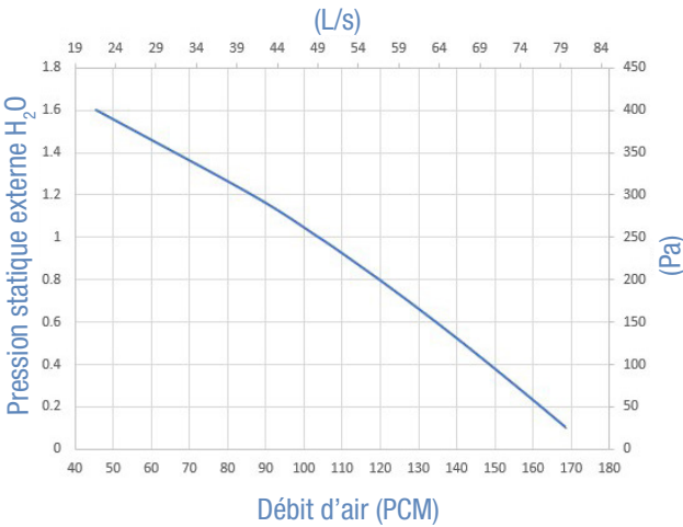
EK150-TF Performance de ventilation
