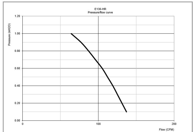
E130-HR-M-N-N Ventilation Performance
