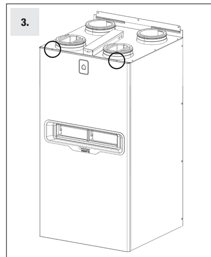
Remove the 2 screws securing the door.
