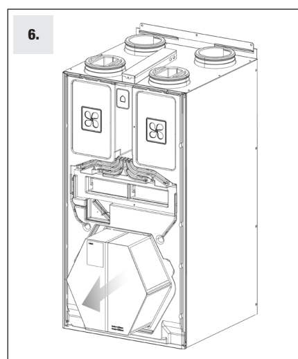
Remove the exchanger by pulling slowly.
