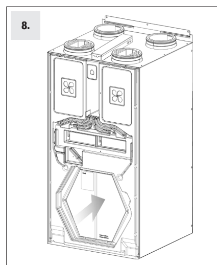
Replace the exchanger by carefully pushing it carefully horizontally.
