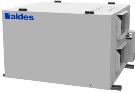
H/E650 models 36 1/4 in (L) x 32 1/8 (W) in x 23 7/8 in (H) (921 mm x 816 mm x 606 mm)
