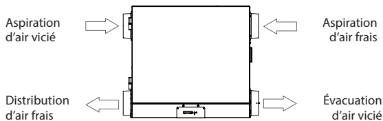
VERSION INVERSEE E130-HRX-N-M
