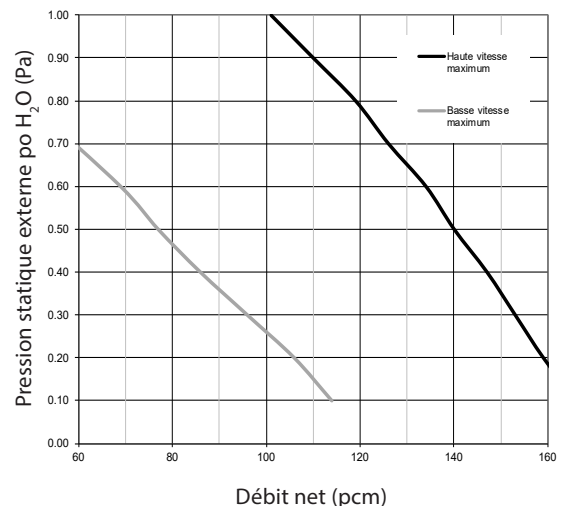
E130-HRX-N Performance de Ventilation
