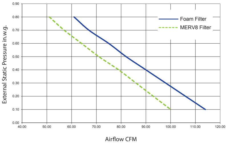
E130-HF-N Ventilation Performance
