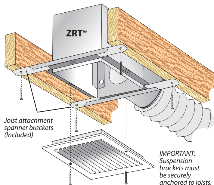
FIGURE 1 - MOUNTING
