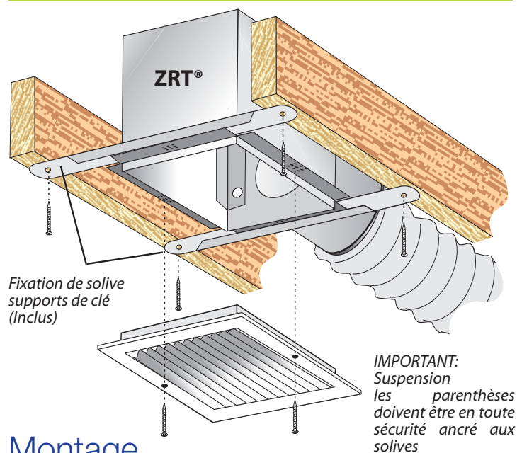
FIGURE 1 - MONTAGE
