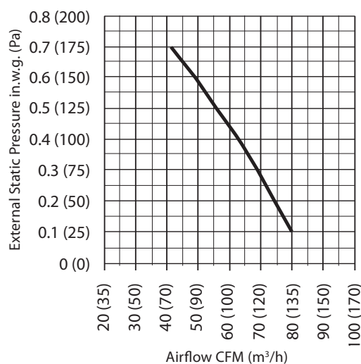
E80-HF-N Ventilation Performance
