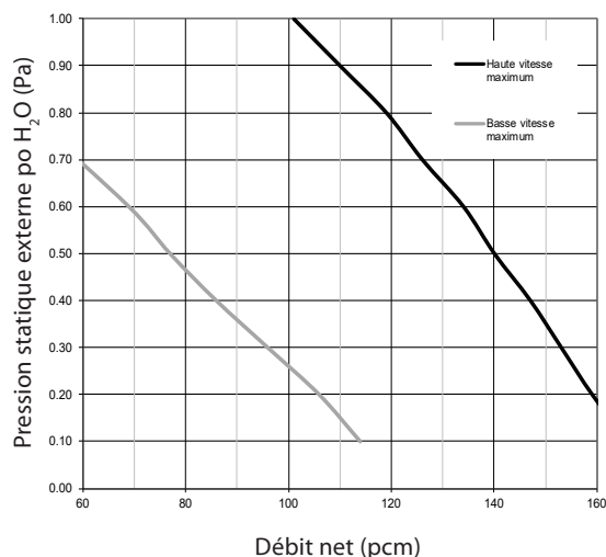
E130-HRX-N Performance de Ventilation
