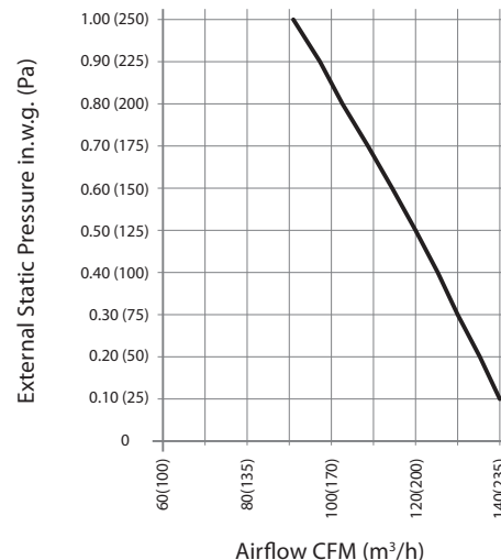
E130-HR-N Ventilation Performance
