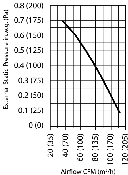
E110-TF Ventilation Performance
