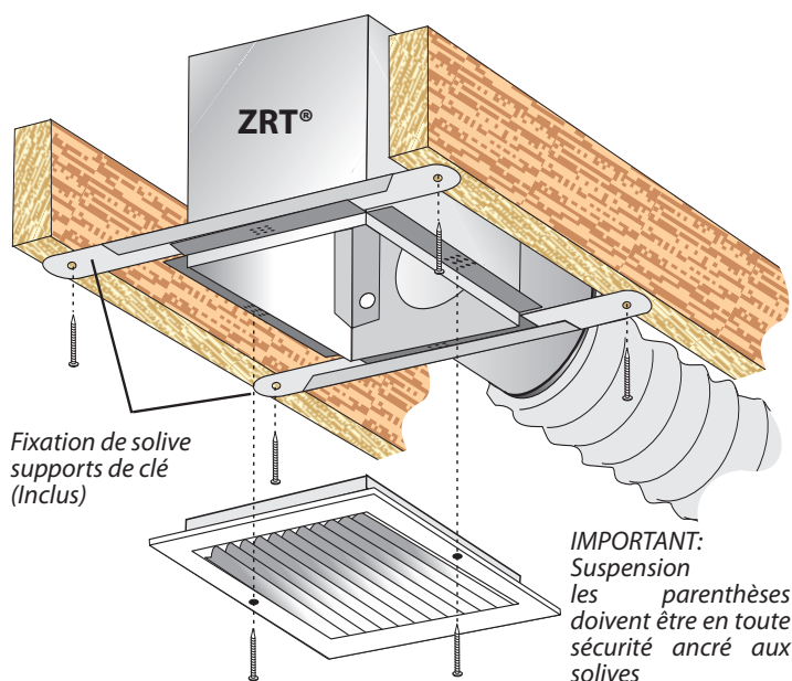
FIGURE 1 - MONTAGE
