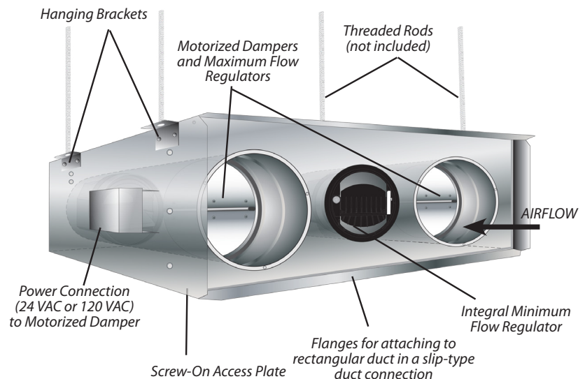
FIGURE 1 - MOUNTING
