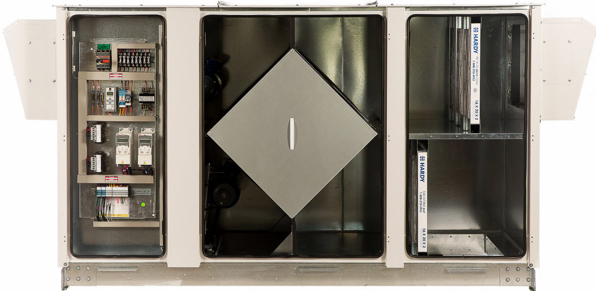
Standard PE outdoor model shown with vertical duct connections..
