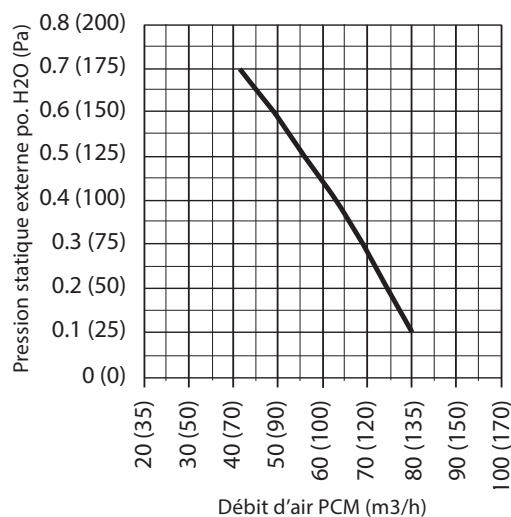
E80-HRG Performance de ventilation
