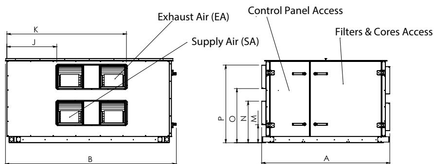
LEFT VIEW
