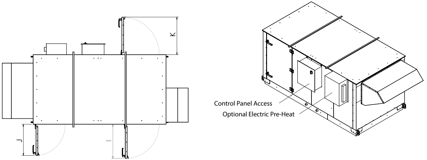
TOP VIEW
