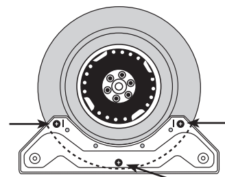
Mounting Bracket and Screw Locations (using the wrong length screws will damage the fan impeller)
