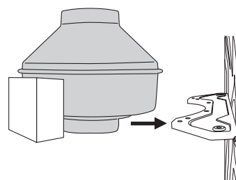
Mount Bracket (use 3/4" long wood screws)
