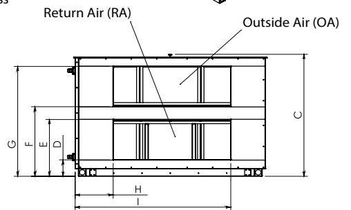
RIGHT VIEW
