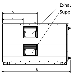
LEFT VIEW
